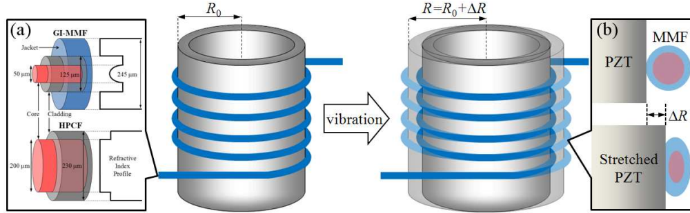
Fig. 1. Schematic diagram of the PZT-fiber assembly. The inset (a) shows the dimensions and their refractive index profiles of the MMFs used in our experiments and their refractive index profiles. The inset (b) shows exaggerated cross-sectional views of the assembly before (upper) and after (lower) stretching.
